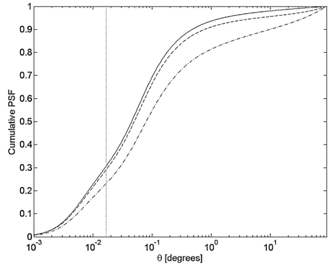
Figure 4. The CIE 1999 total glare function (PSF) integrated from the center (0 degrees) outwards, for the same age/pigmentation conditions as in Figure 2. At 90 degrees the integrated value is 1 by definition, since the PSF is normalized. For angles smaller than 90 degrees, the fraction of light up to that angle in the PSF is indicated. The fraction of light in the central part of the PSF, below 1 minute of arc (dotted line) that determines visual acuity is only about 30%.
