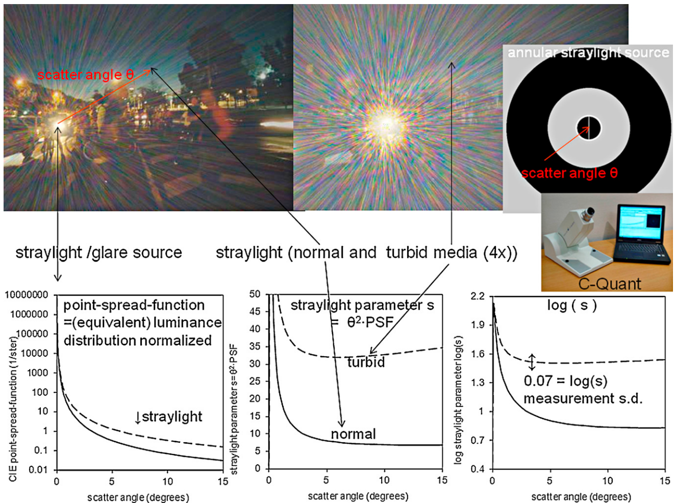
Figure 1. Basics of straylight quantification. At the top a street scene is depicted as it would be seen by an eye with normal straylight (left), and by an eye with 4x increased straylight (right). The 3 figures at the bottom give the point-spread-function according to the CIE for average age-best eyes. The PSF is given using 3 corresponding definitions: the normal (left), the straylight parameter s linearly (middle), and the same logarithmically (right). The continuous line is for an average 35-year-old Caucasian eye; the dashed line is for a caucasian eye with media turbidity increasing straylight 4x, mimicked using the CIE function for a 95-year-old. At the top right the stimulus lay-out is shown as used in the C-Quant.
