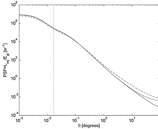
Figure 2. The CIE 1999 total glare function for a 35-year-old negroid (continuous line), a 35-year-old blue-green eyed Caucasian (dashed line) and a 80-year-old blue-green eyed Caucasian (dash-dotted line). The vertical dotted line indicates 1 minute of arc. This is customarily assumed to be the smallest detail that can be resolved by an eye having a visual acuity of decimal 1.
