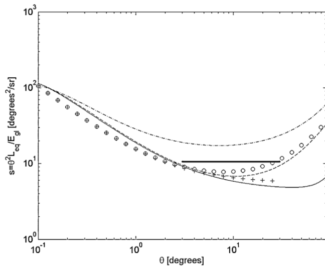
Figure 5. The simplified versions of the total glare equation of a 35-year-old blue-green eyed Caucasian. The age adapted Stiles Holladay equation is shown with the thick line, the simplified glare equation as +, and the general glare equation as o. For clarity also the total glare function is plotted for a 35-year-old negroid (continuous line), a 35-year-old blue-green eyed Caucasian (dashed line) and a 80-year-old blue-green eyed Caucasian (dash-dotted line).
