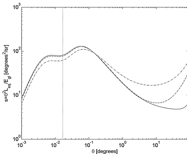
Figure 3. The CIE 1999 total glare function (PSF) multiplied by \theta^2 to represent it in terms of the straylight parameter for the same age/pigmentation conditions as in Figure 2 (Reprint with permission of encyclopedia of the eye, Darlene A. Dartt ed.).
